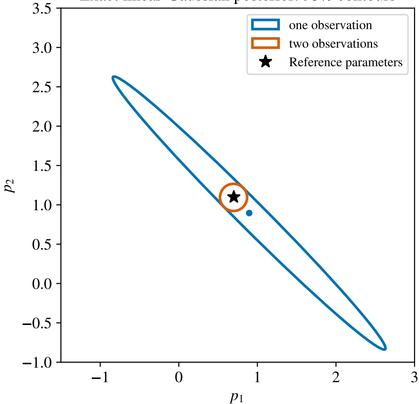
Exact linear-Gaussian posterior: 95% contours
