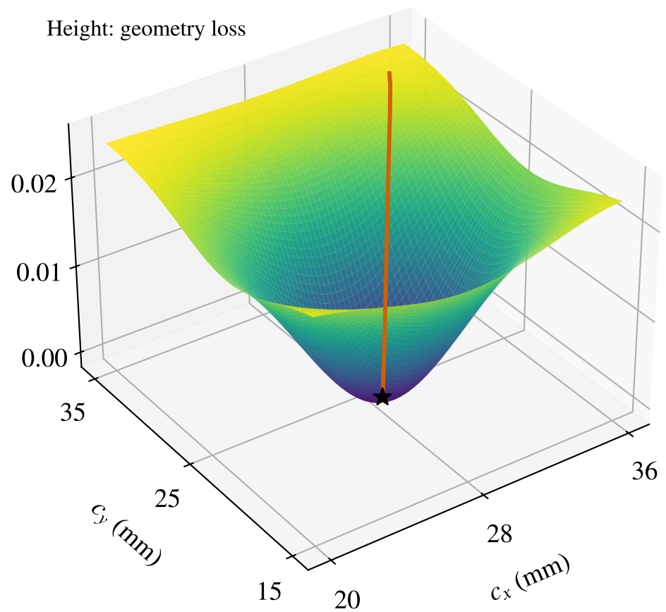
(a) A computed loss surface
