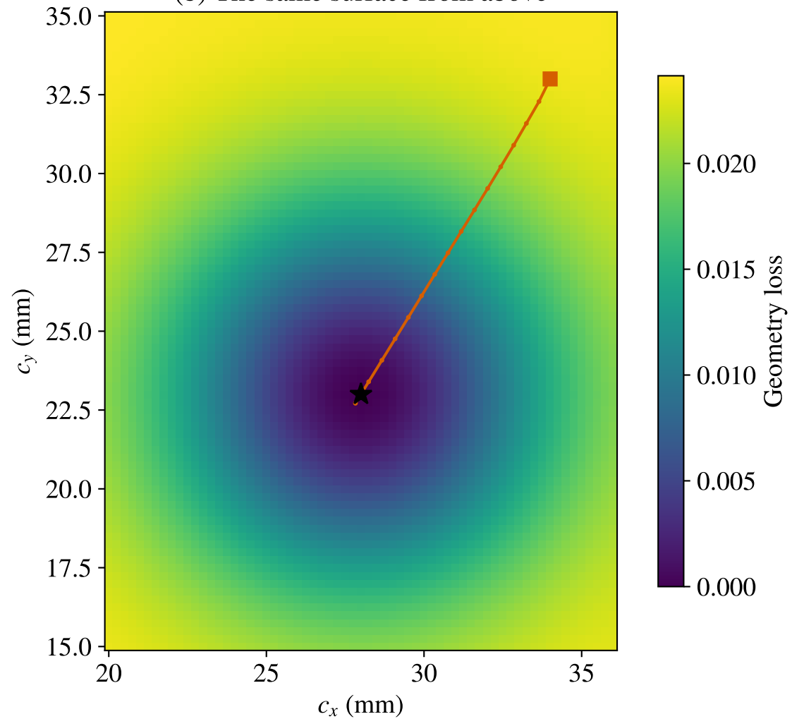
(b) The same surface from above
