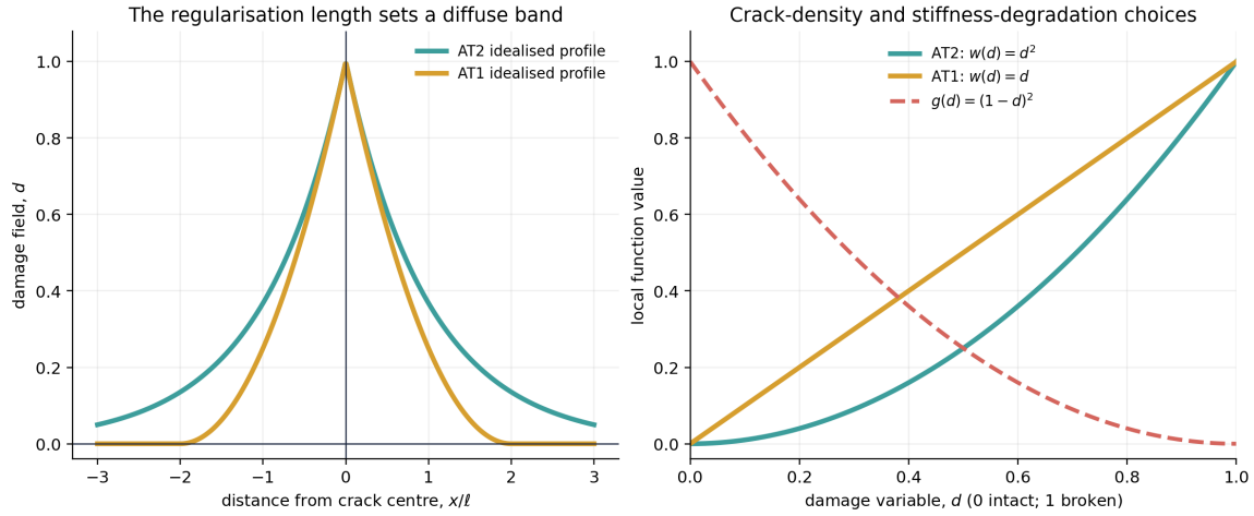
Fig. 9.1: The crack-density choice and the stiffness degradation law are independent mathematical functions. Together, they govern how damage nucleates, diffuses, and softens the solid.
