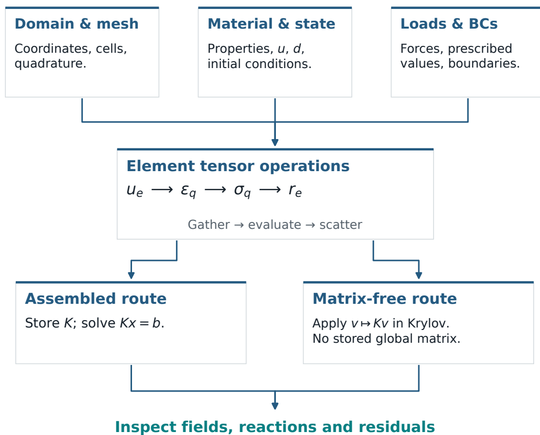
Fig. 11.1: The finite element pipeline translates physical boundary-value problems into discrete tensor operations, connecting continuous weak forms to PyTorch data structures.
