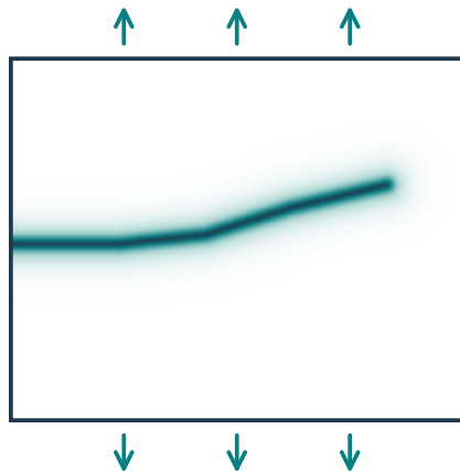
Diffuse phase field
