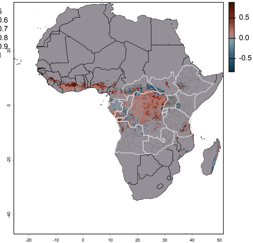
Ebola ecological niche - difference
