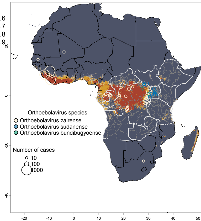
Ebola ecological niche (2026 Data) & recorded outbreaks
