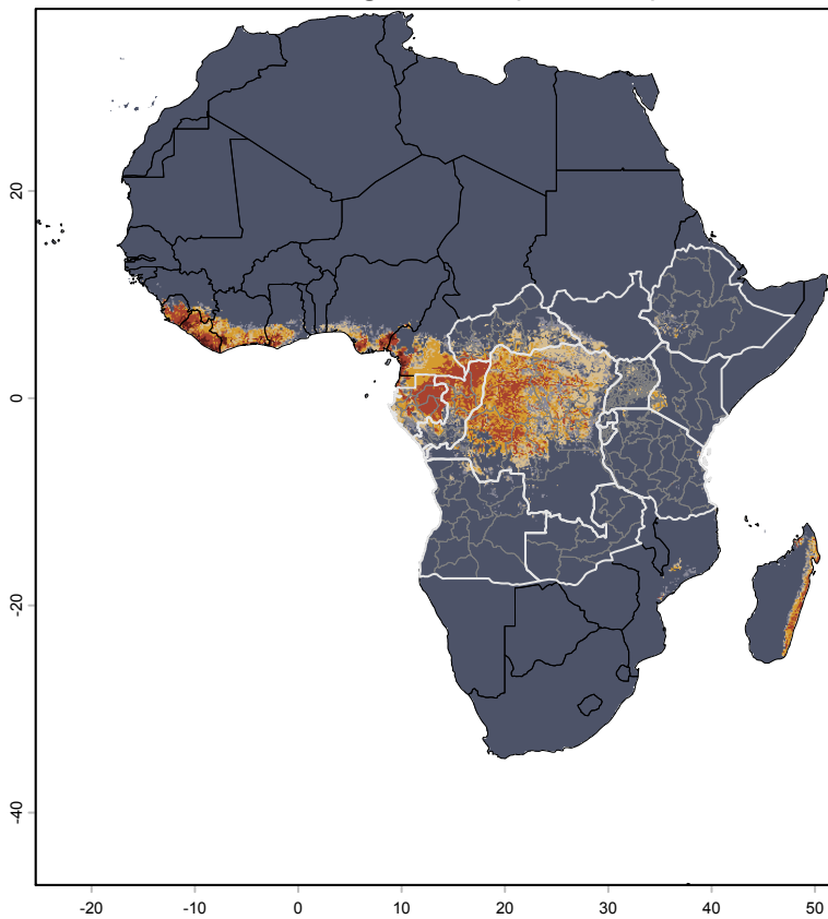
Ebola ecological niche (2016 Data)
