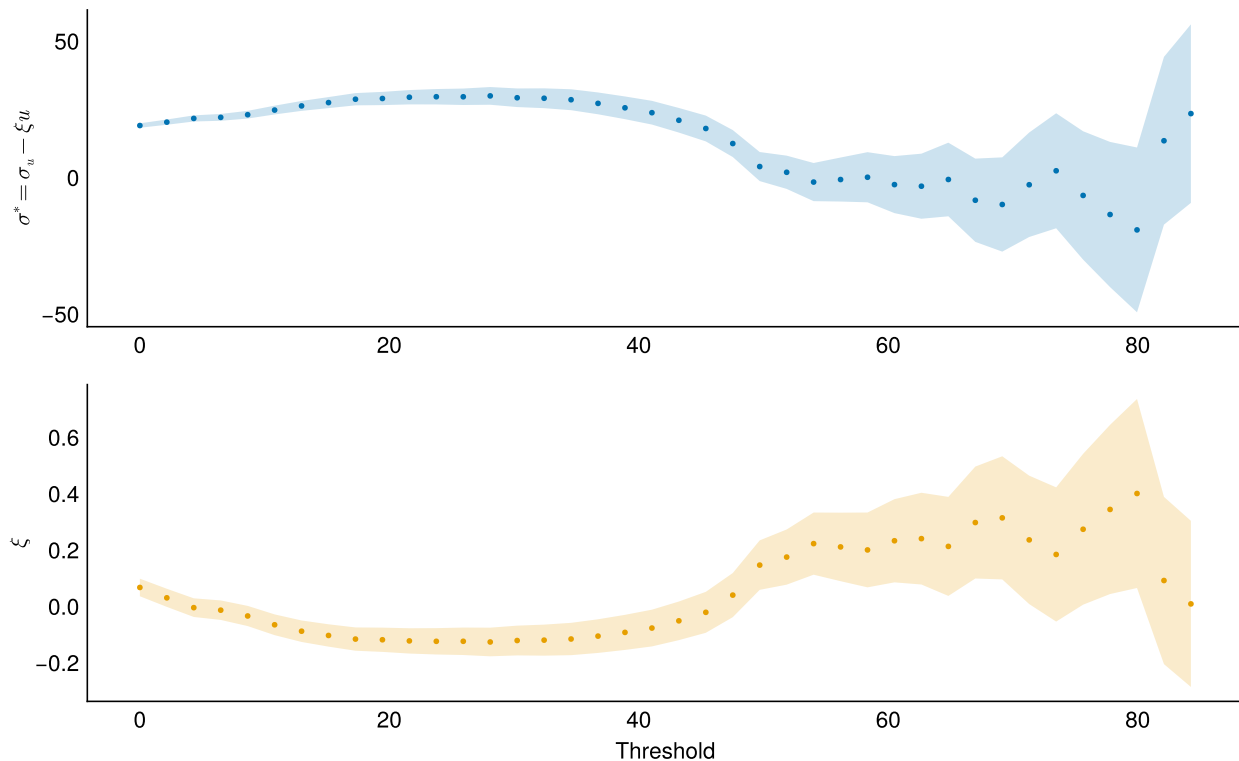
Figure 2: Parameter stability plot.
