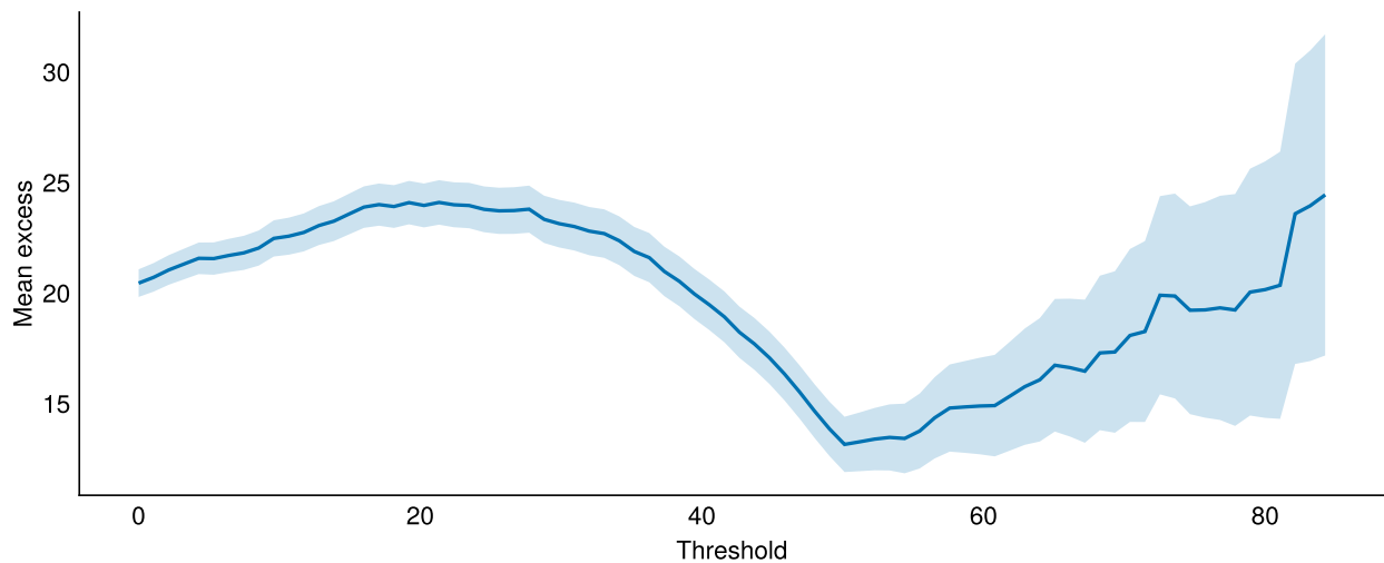
Figure 1: Mean residual life plot.
