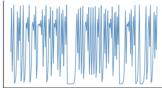
r = 4.0 (chaos)
