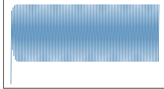
r = 3.2 (period 2)
