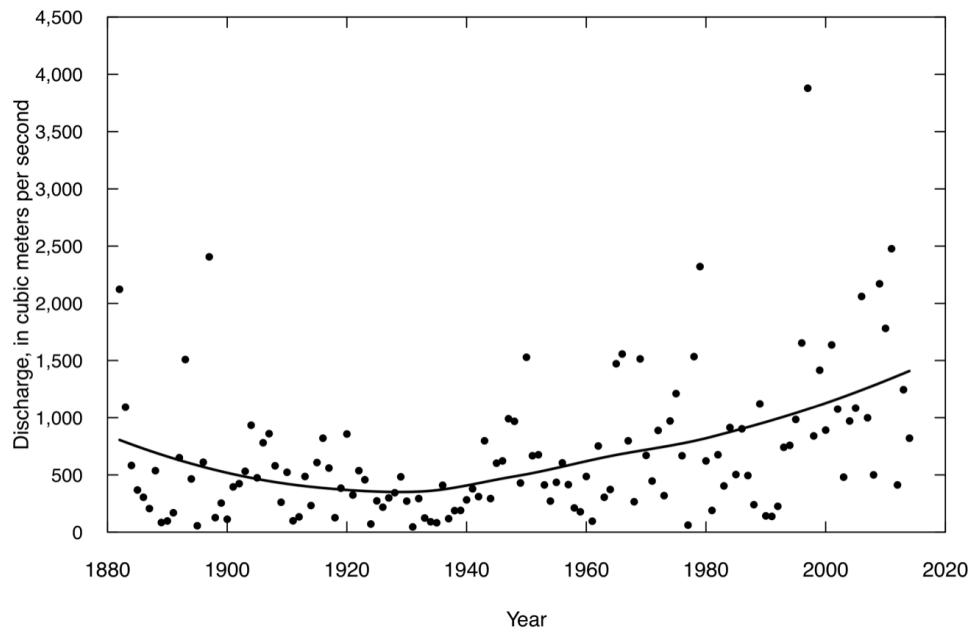
Figure 12.17. Graph of annual peak discharge, Red River of the North, at Grand Forks, North Dakota, 1882–2014, and a loess smooth of the data (using the default span value of 0.75).
