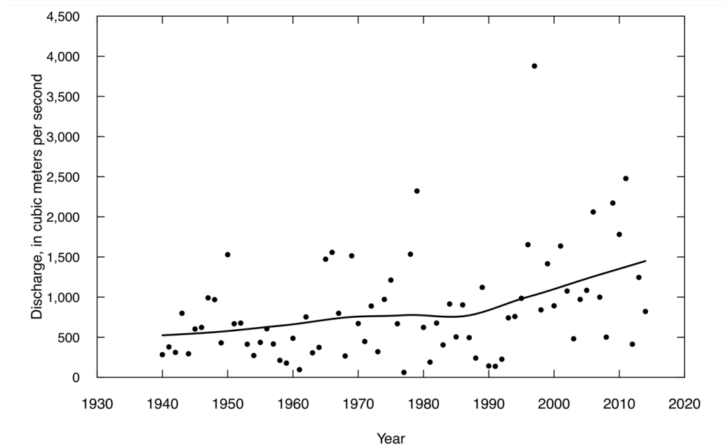
Figure 12.16. Graph of annual peak discharge, Red River of the North, at Grand Forks, North Dakota, 1940–2014, and a loess smooth of the data (using the default span value of 0.75).
