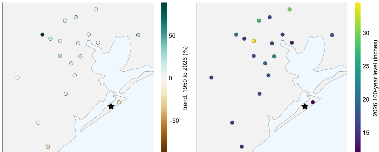
Figure 2: Each station fit to its own record. Left: trend, as the percent change in every return level from 1950 to 2026. Right: 100-year daily rainfall in 2026. Scholes Field is the star.
