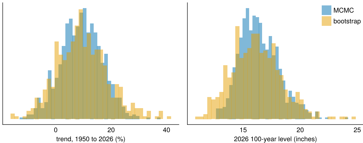
Figure 3: The pooled fit at Scholes Field by MCMC and by the bootstrap over years. Left: trend. Right: 2026 100-year level.
