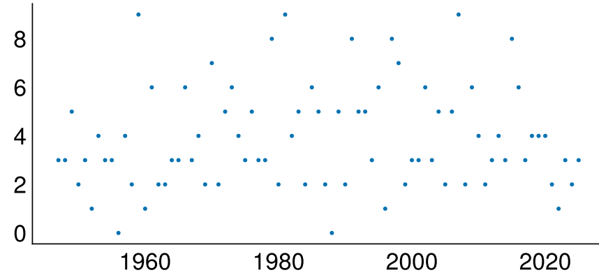
Storms per year: Mann-Kendall p = 0.50
