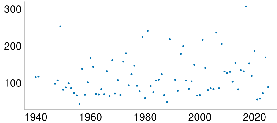
Largest day each year (mm): Mann-Kendall p = 0.19
