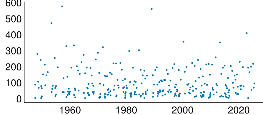
Days since the previous storm: Mann-Kendall p = 0.90
