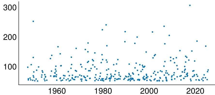
Largest day of each storm (mm): Mann-Kendall p = 0.42
