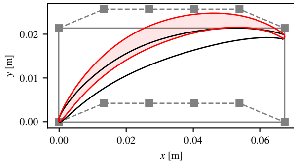
c) Upper bound deformation
