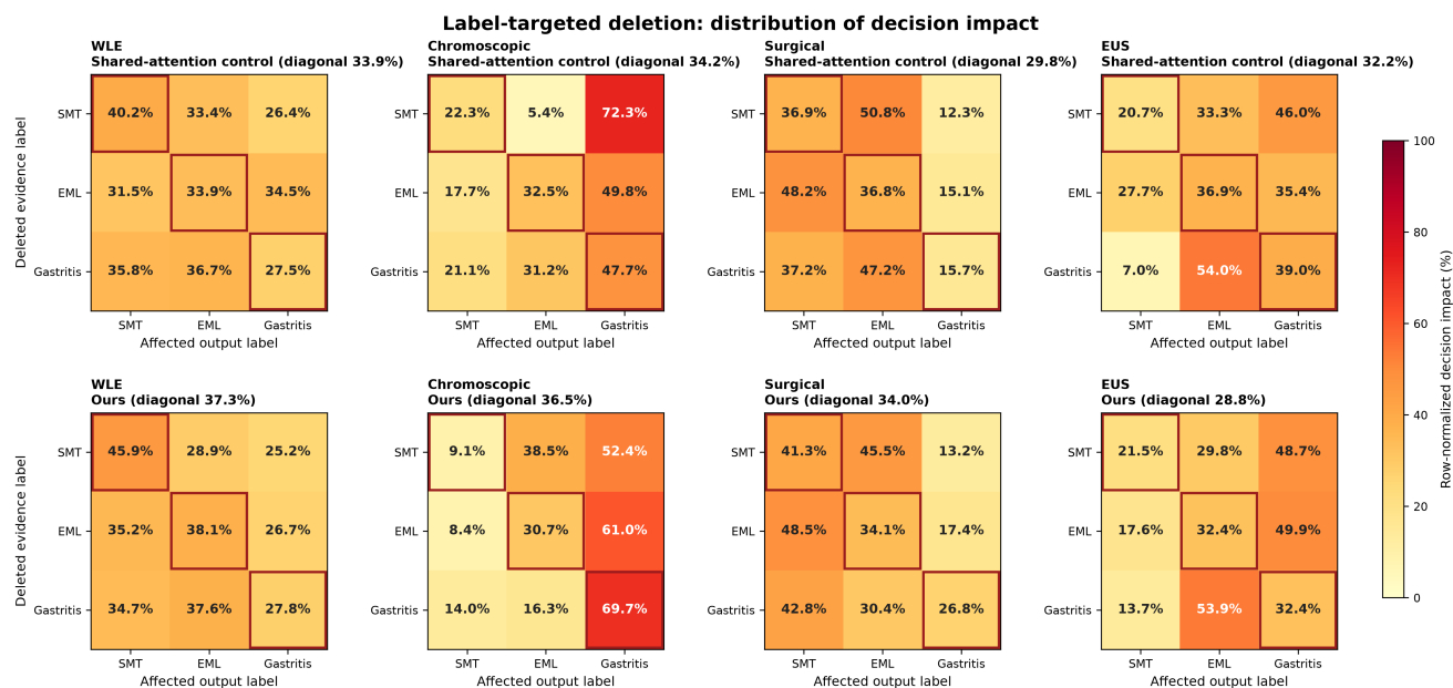
Top-5 evidence deletion before hypergraph reasoning; rows sum to 100%; stronger diagonal concentration indicates greater label selectivity
