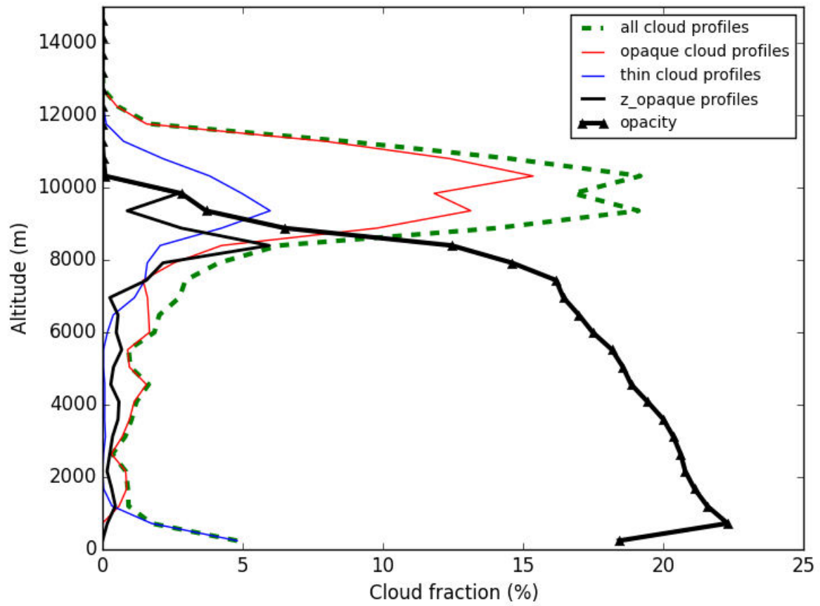
Cloud and z_opaque fraction (%) mean profiles for CALIPSO COSPv2.0
