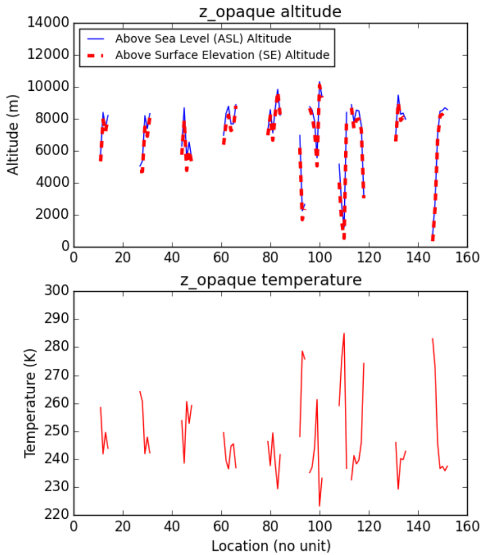
CALIPSO z_opaque variables COSPv2.0 : Altitude_ASL, Altitude_SE and Temperature
