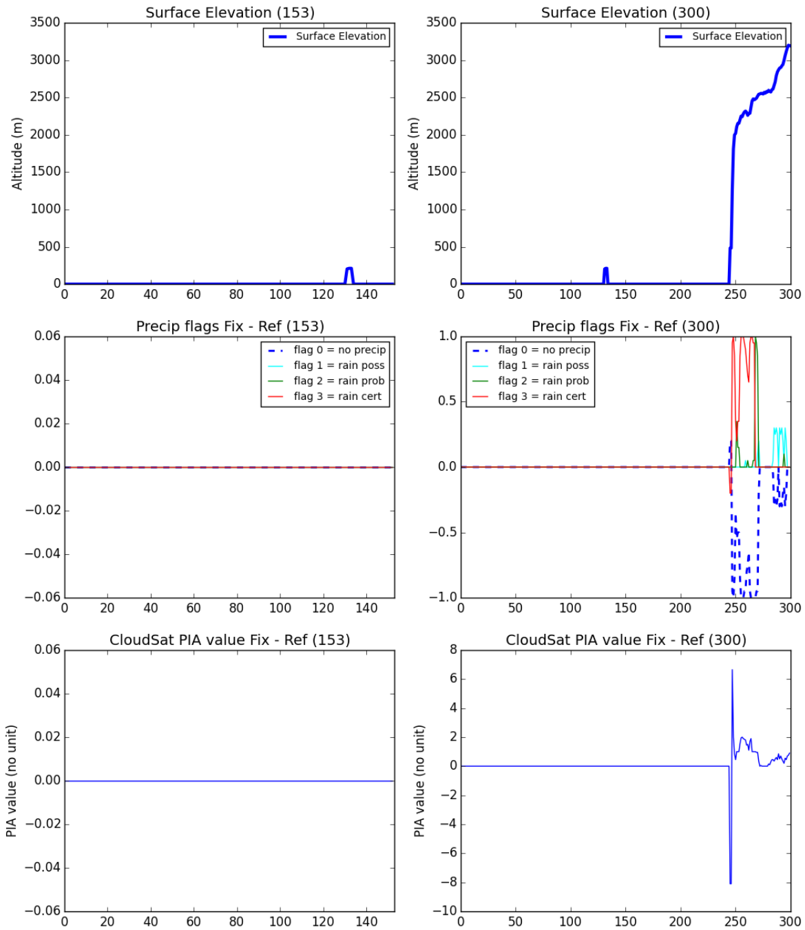
Debugging Precip Flag and PIA diagnostics for COSPv2.1 CloudSat simulator (Fig.2)
