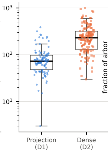
Branch points AUC = 0.89
