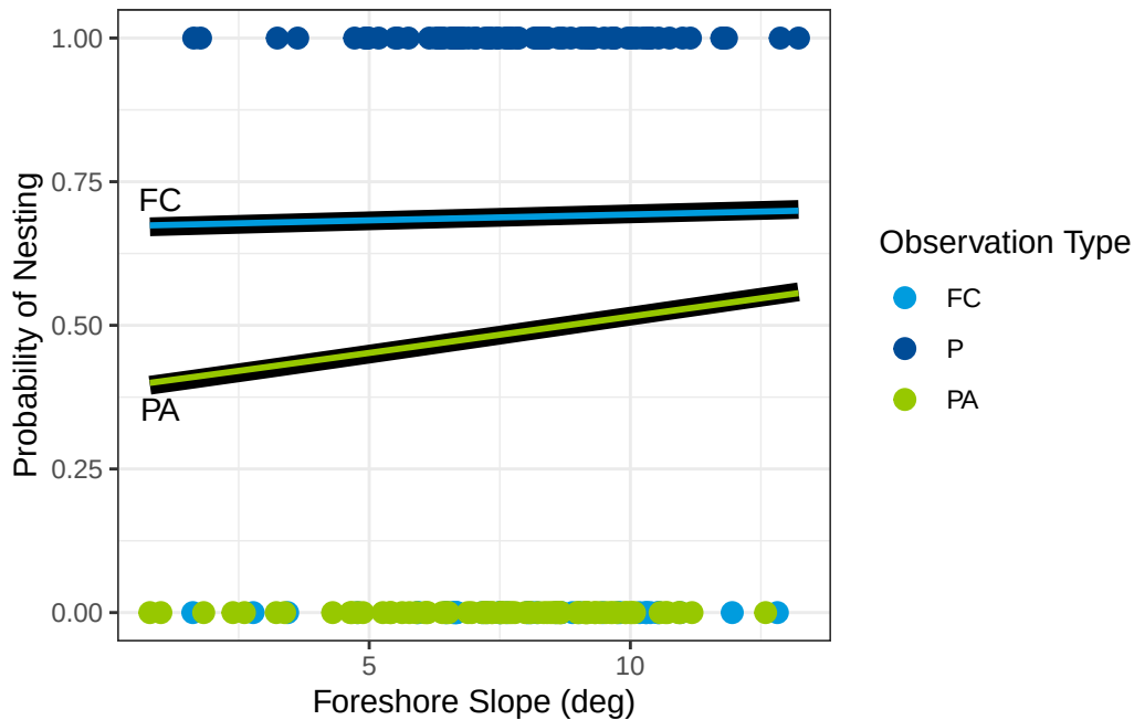
Figure 2.1: Probability of Nesting vs. Foreshore Slope
