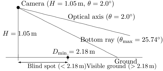
Figure 2. Geometric optical projection illustrating the physical near-field blind spot ( D_{\min} = 2.178 m) where ground-contact lines fall below the camera’s vertical field of view.
