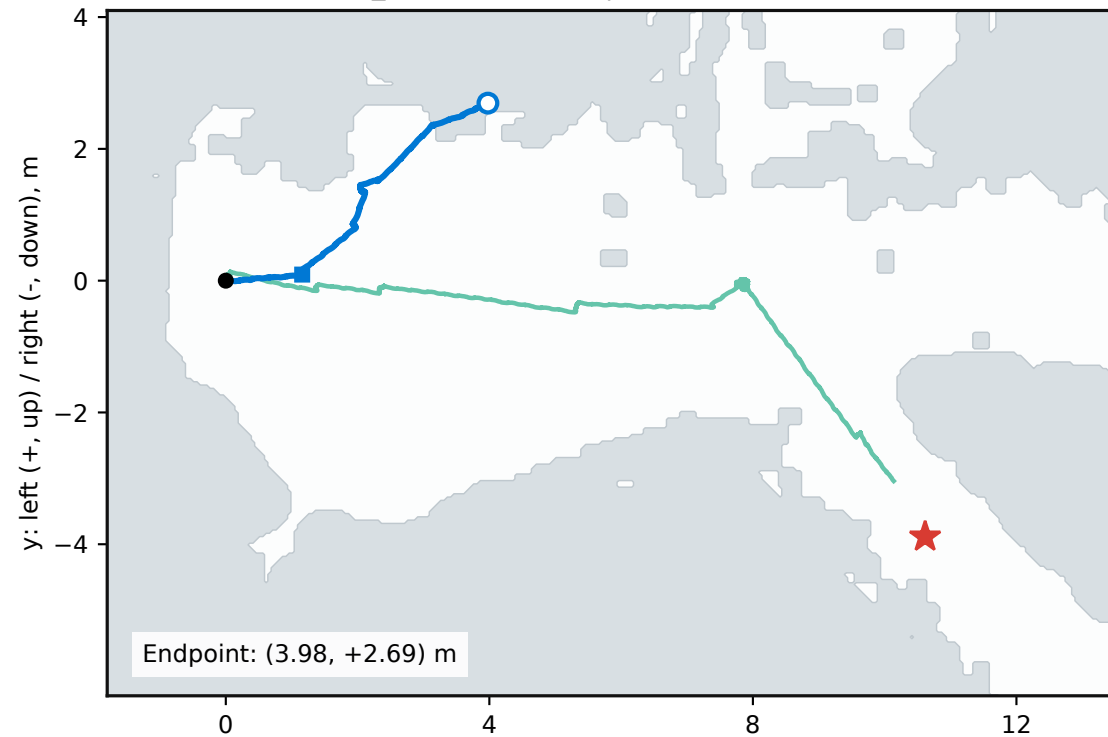
x: forward from marked start (m) First turn: command +30°, odom +28.31°, body IMU +28.33°
