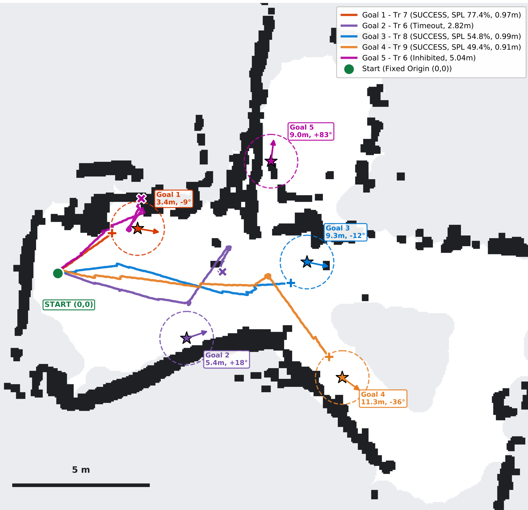
Unitree Go2 VLM Navigation Trajectories Across 5 Goal Poses (Paper Fig. 6)
