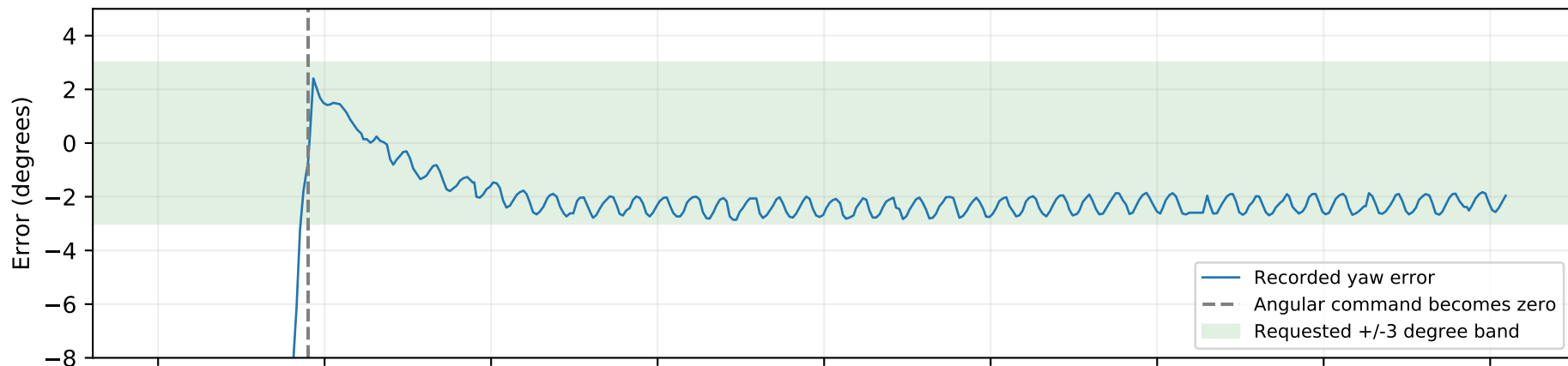
New goal 5: angle reached; zero command persists until motion timeout
