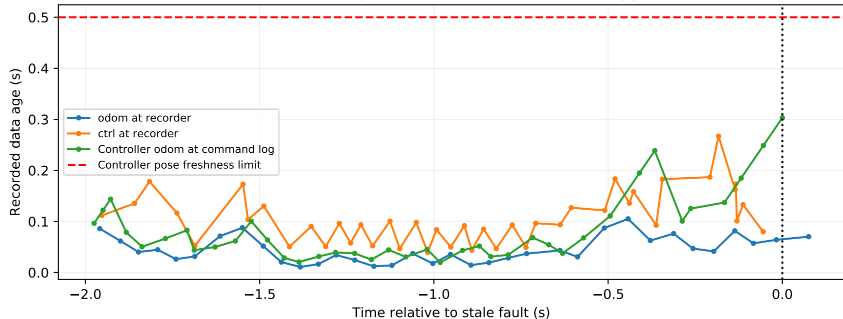
Latest control pose inside controller was not logged
