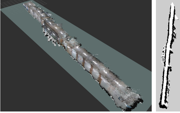
Fig. 4. Visual mapping results from real-world deployment. Left: Reconstructed 3D point cloud map from RTAB-Map. Right: Projected 2D occupancy grid map.
