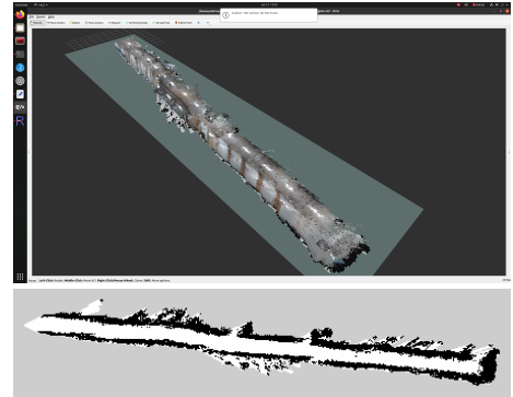
Fig. 2. Visual SLAM mapping results inside the Oseok Hall corridor. (a) Reconstructed 3D point cloud map. (b) Projected 2D occupancy grid map used for path planning and navigation.
