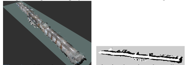
Fig. 4. Visual mapping results in the virtual sandbox. Left: Reconstructed 3D point cloud map from RTAB-Map. Right: Projected 2D occupancy grid map.
