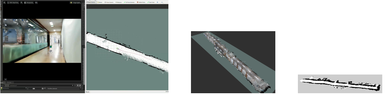
Fig. 3. Simulation validation results in the virtual sandbox. (a) Nav2 navigation stack active in the 3DGS environment, showing the simulated quadruped in Isaac Sim (left) and path planning/costmap in RViz (right). (b) Reconstructed 3D point cloud map from RTAB-Map. (c) Projected 2D occupancy grid map.
