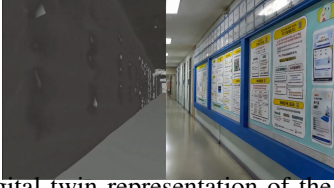
Fig. 2. Digital twin representation of the campus corridor. Left: Sparse volumetric collision mesh generated using fVDB. Right: High-fidelity photorealistic 3DGS render.
