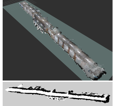
Fig. 2. Visual SLAM mapping results inside the Oseok Hall corridor. (a) Reconstructed 3D point cloud map. (b) Projected 2D occupancy grid map used for path planning and navigation.
