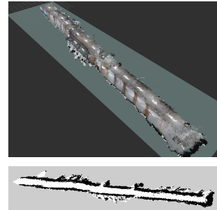
Fig. 4. Visual mapping results in simulation. Top: Reconstructed 3D point cloud map from RTAB-Map. Bottom: Projected 2D occupancy grid map.
