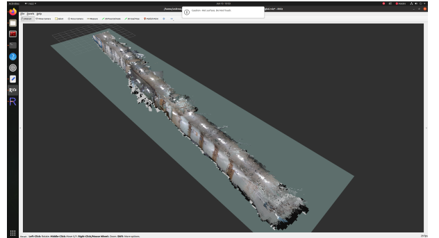
Fig. 2. Visual SLAM and path planning validation inside the reconstructed 3DGS corridor environment. The reconstructed mesh provides accurate collision responses and realistic visual feedback.
