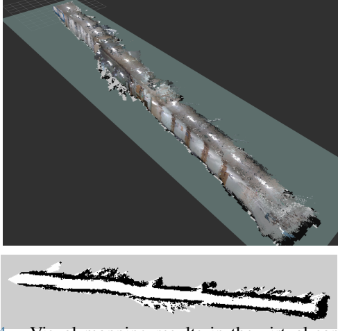
Fig. 4. Visual mapping results in the virtual sandbox. Top: Reconstructed 3D point cloud map from RTAB-Map.
