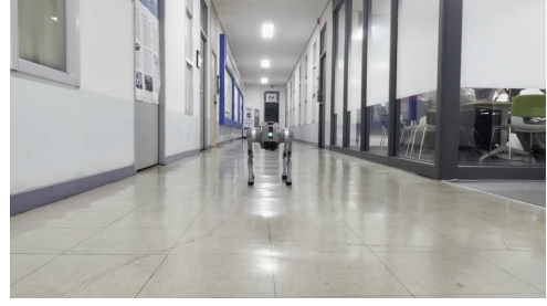
Fig. 5. Real-world experimental setup. The Unitree Go2 robot is equipped with an Intel RealSense D435i and Jetson Orin NX, running the entire navigation stack on-board.
