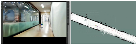
Fig. 3. Autonomous navigation execution inside the reconstructed virtual environment, showing the simulated quadruped robot in Isaac Sim (left) and path planning/costmap synchronization in RViz (right).
