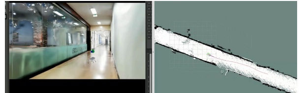
Fig. 3. Autonomous navigation execution inside the reconstructed virtual environment, showing the simulated quadruped robot in Isaac Sim (left) and path planning/costmap synchronization in RViz (right).
