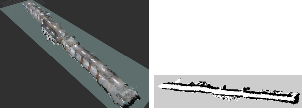
Fig. 4. Visual mapping results in simulation. Left: Reconstructed 3D point cloud map from RTAB-Map. Right: Projected 2D occupancy grid map.
