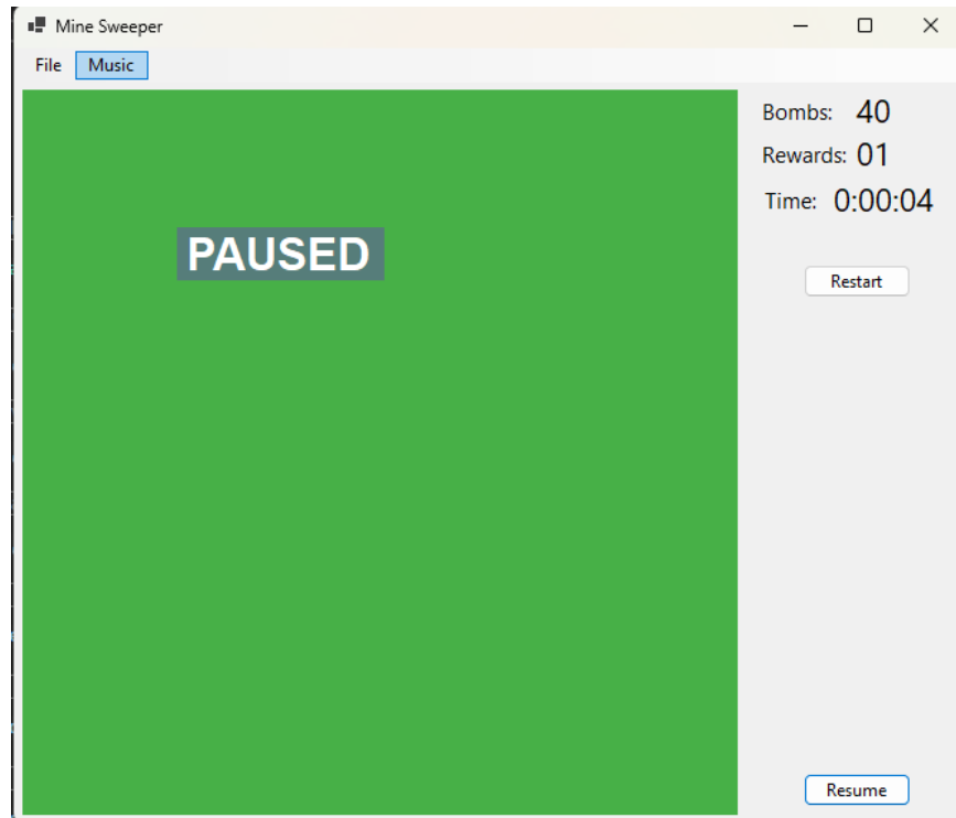
Figure 5: Screenshot of a new 20 x 20 game. While it is paused. The paused label bounces around the screen and the panel and label change colors as it moves around the screen.
