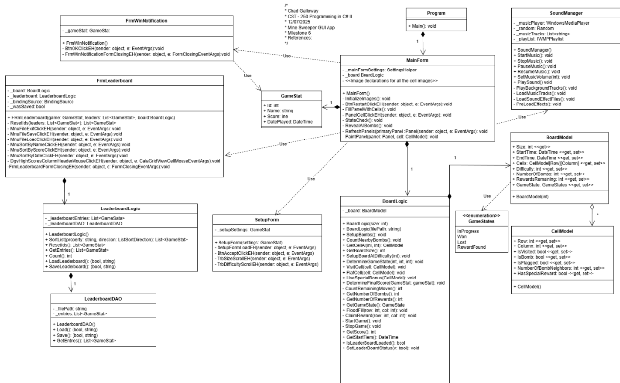
Figure 2: UML Class Diagram for Milestone 6
