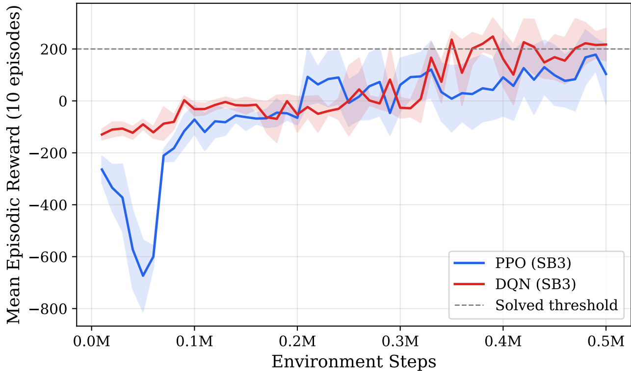
LunarLander-v3: PPO vs DQN Learning Curves
