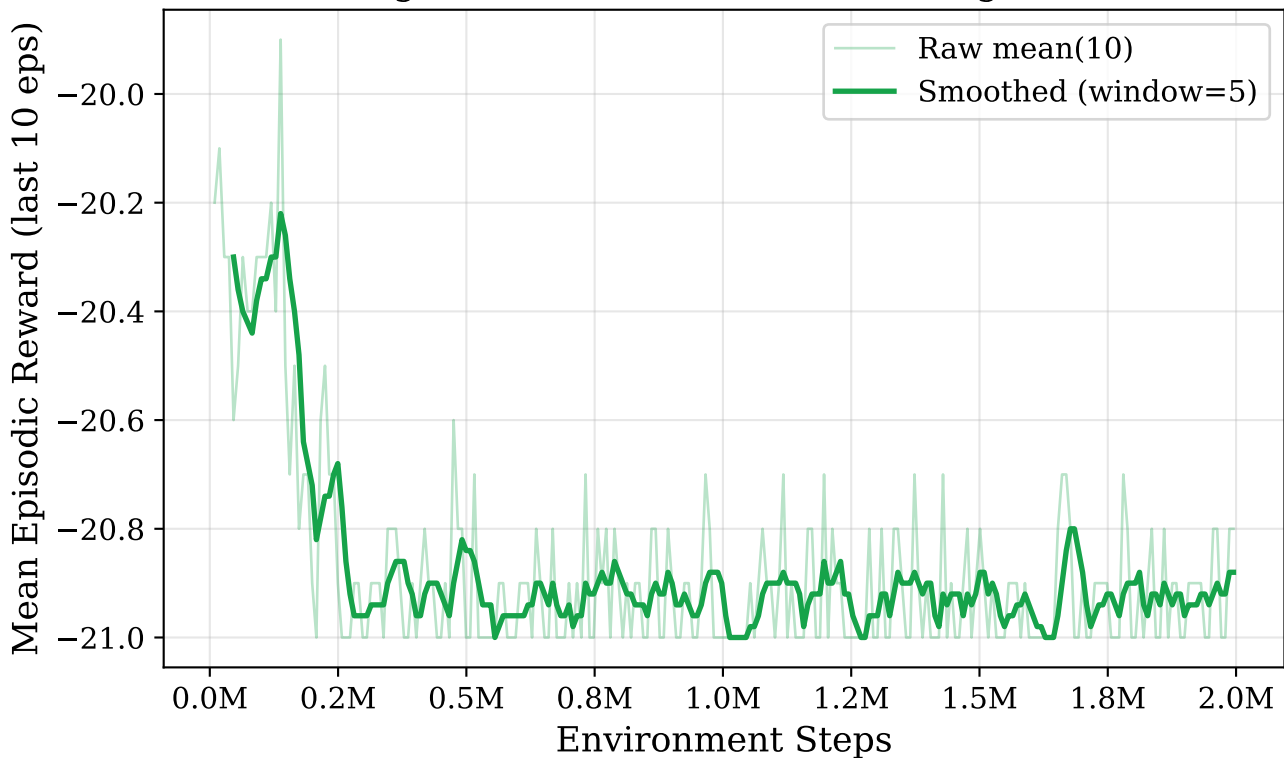
Pong: DQN (from scratch) Learning Curve
