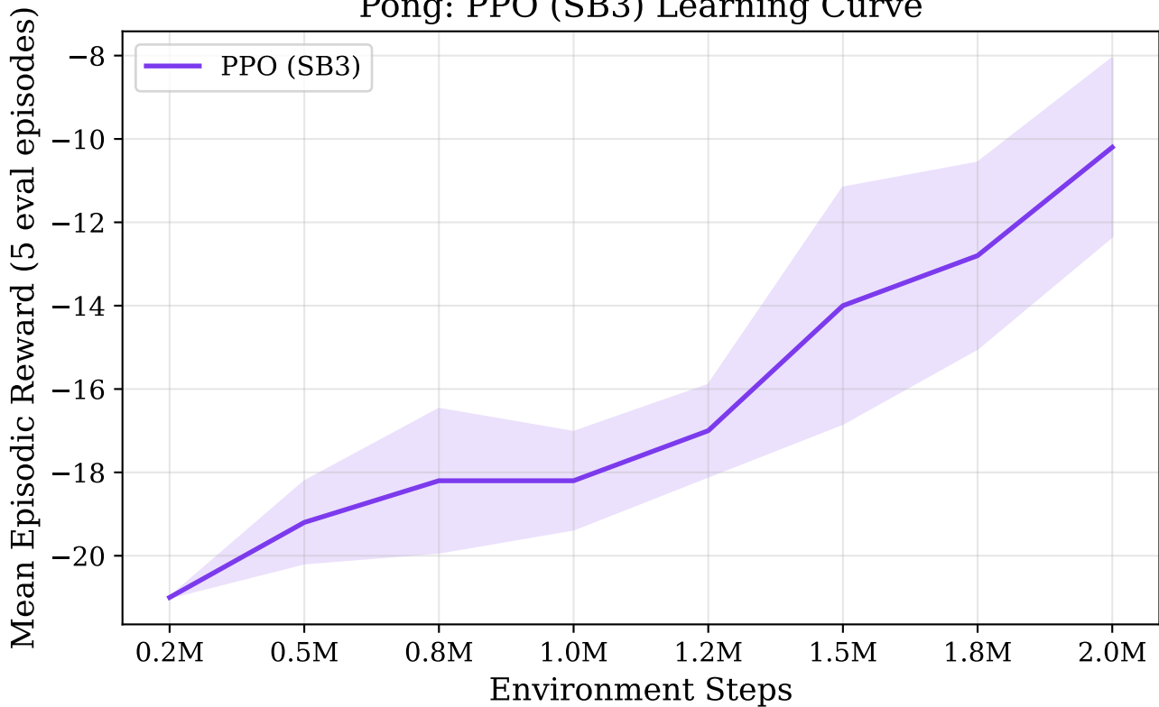
Pong: PPO (SB3) Learning Curve
