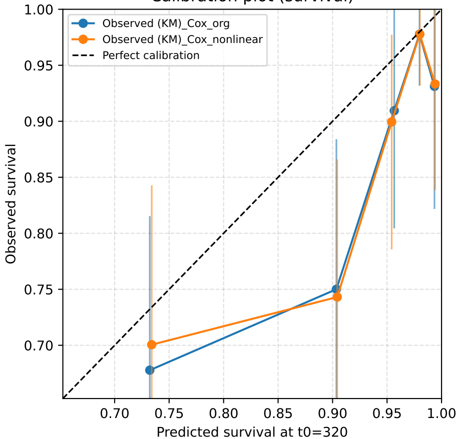
Calibration plot (survival)
