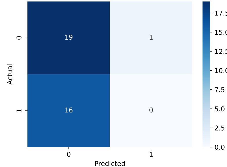
Isolation Forest
