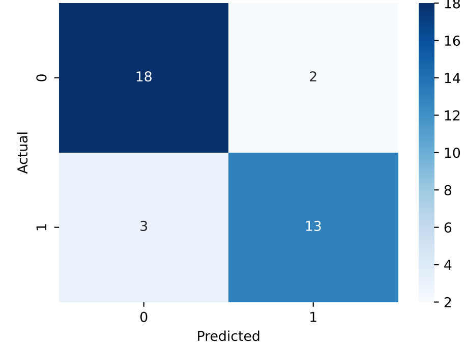
One-Class SVM
