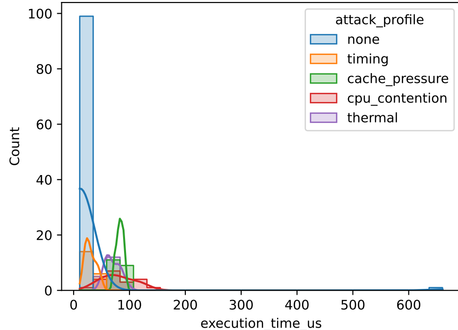
Distribution: execution_time_us
