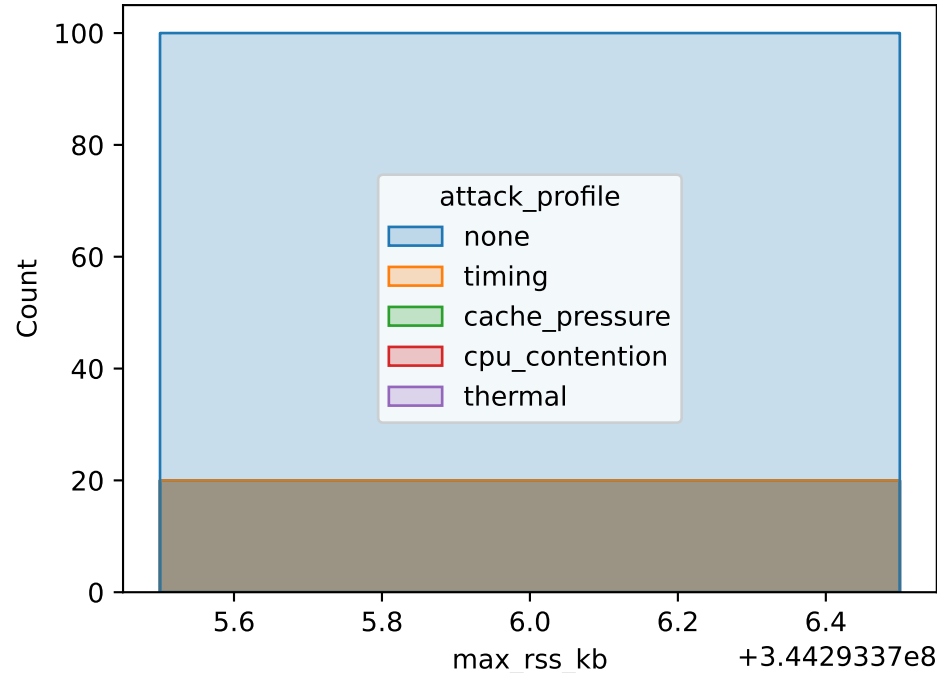
Distribution: max_rss_kb
