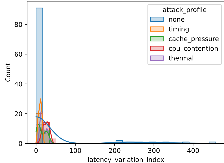
Distribution: latency_variation_index
