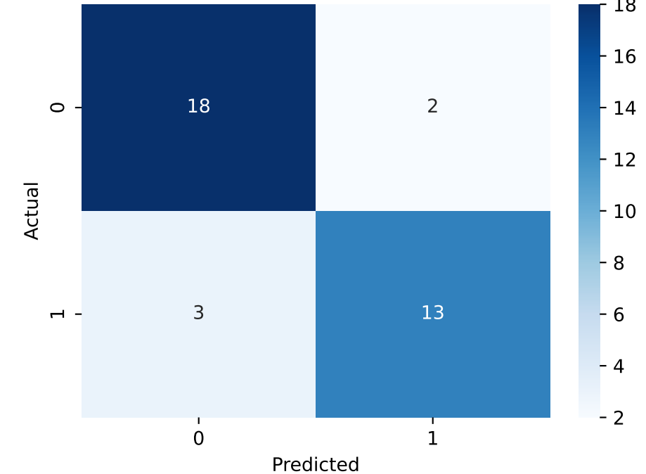
One-Class SVM
