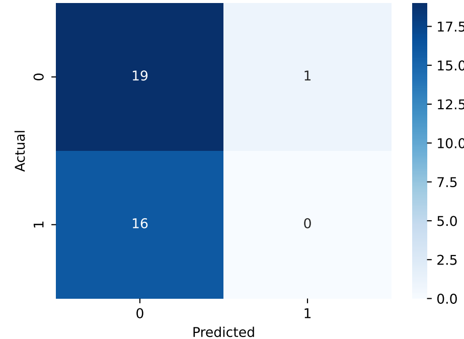
Isolation Forest
