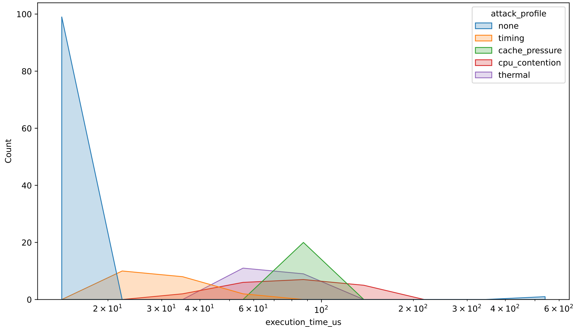
Execution Latency Distribution (Log Scale)
