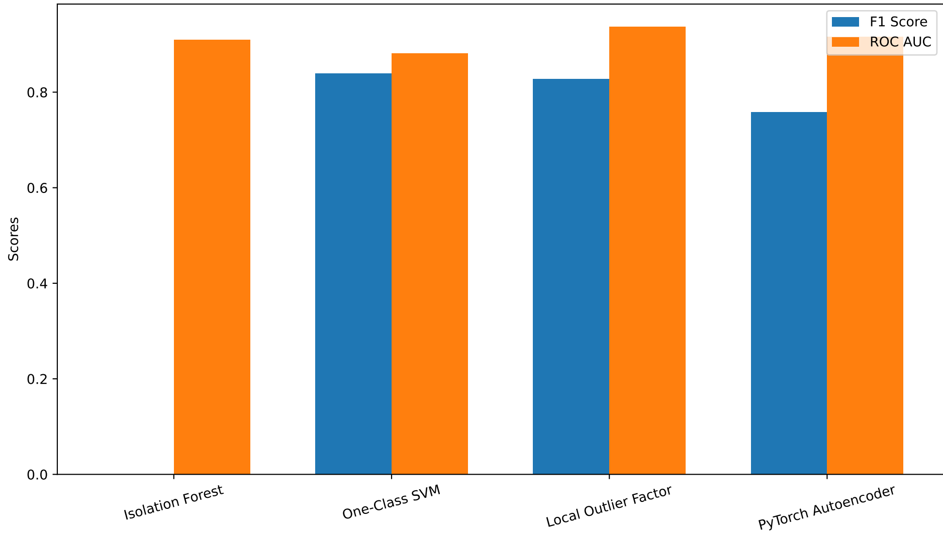
Model Comparison
