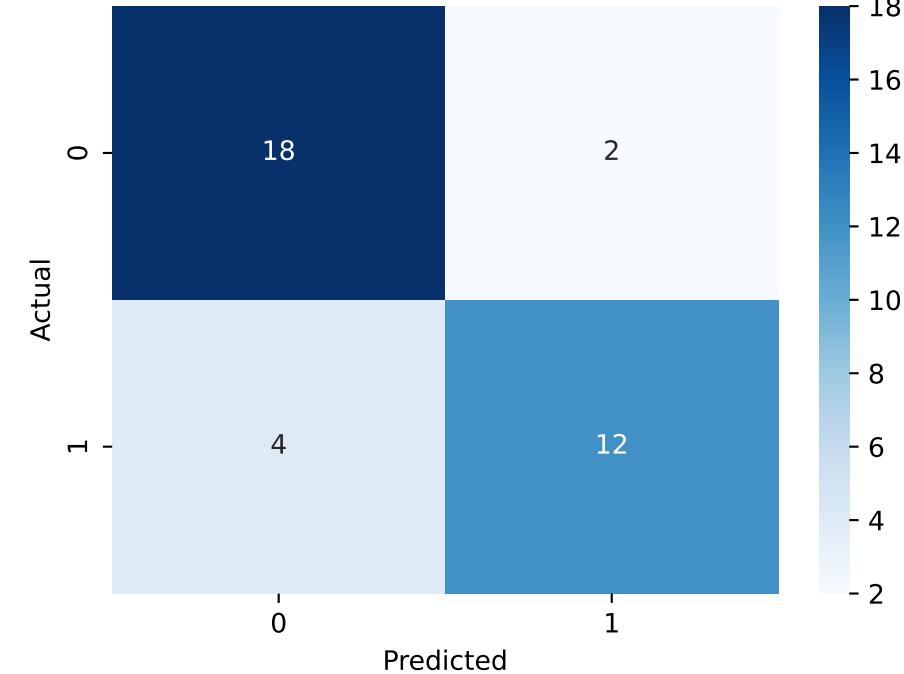
One-Class SVM
