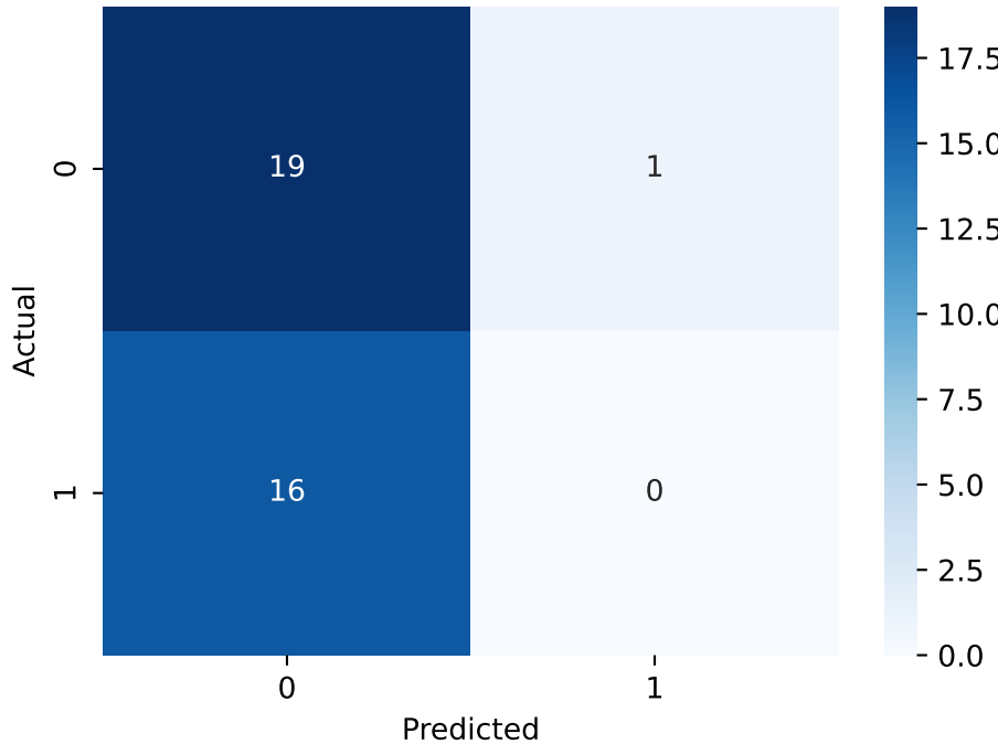
Isolation Forest
