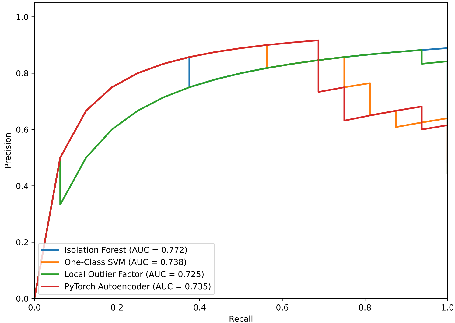
Precision-Recall Curve
