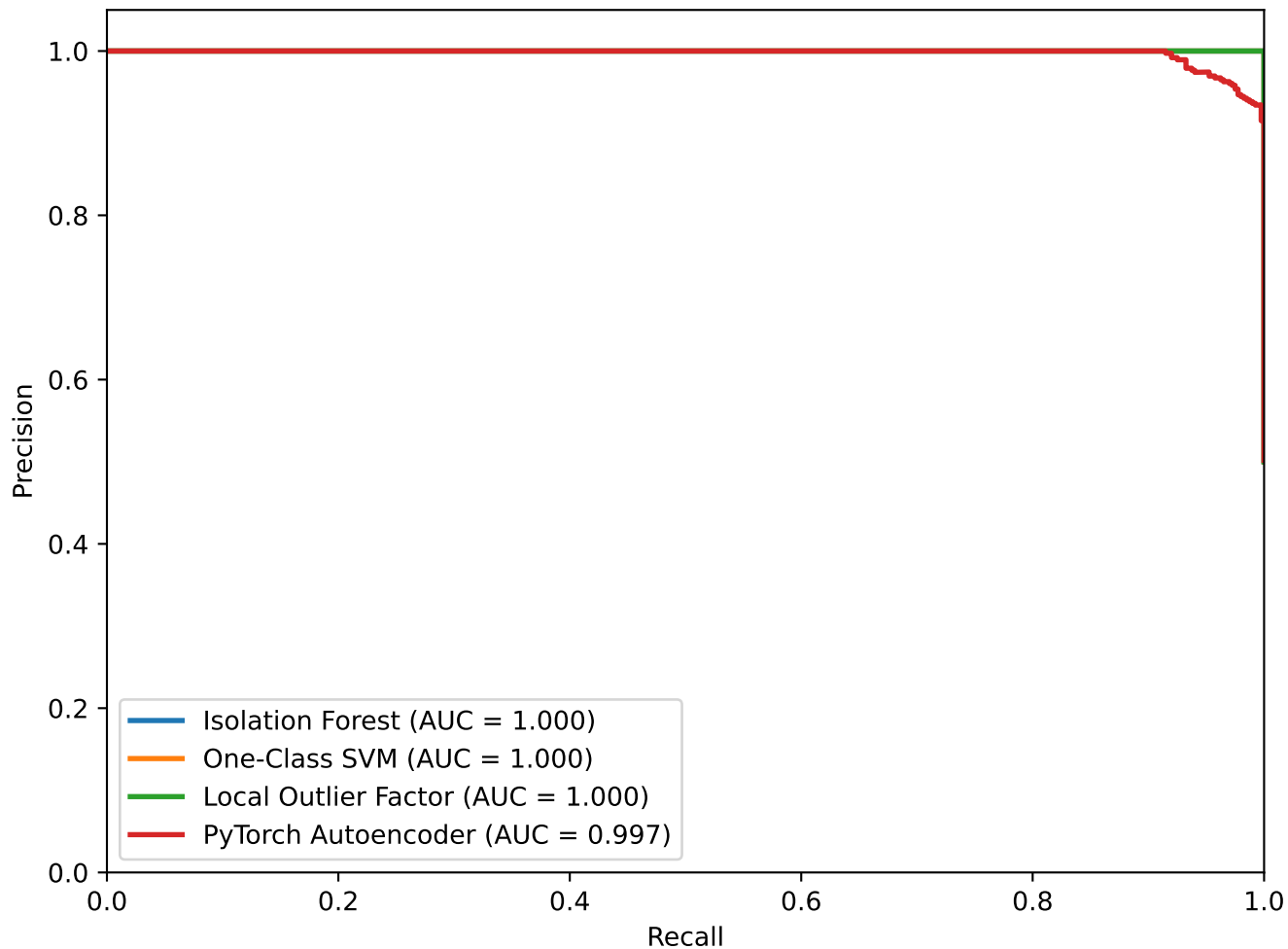
Precision-Recall Curve
