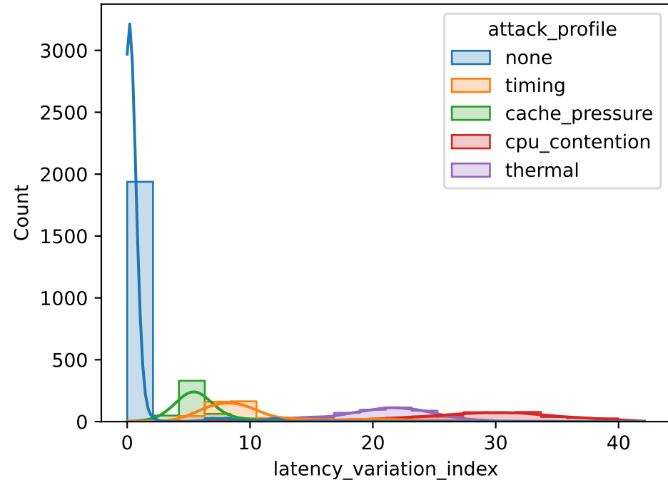
Distribution: latency_variation_index
