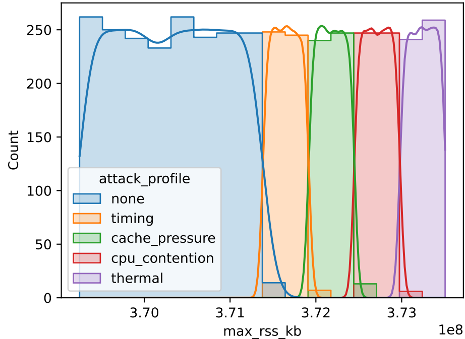
Distribution: max_rss_kb
