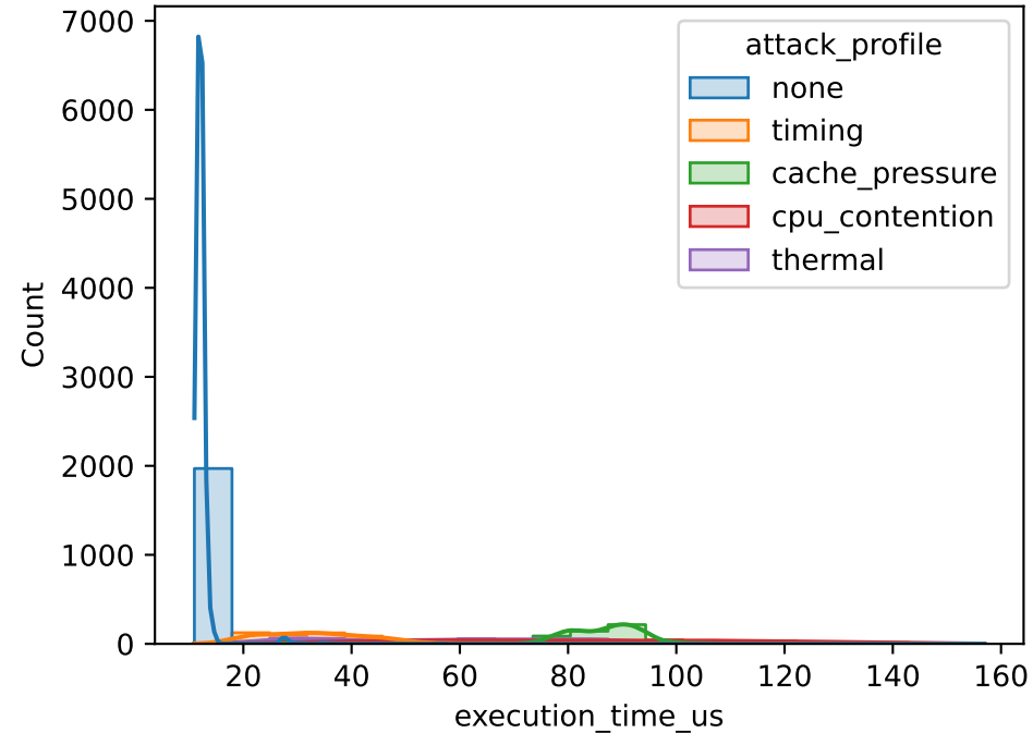
Distribution: execution_time_us
