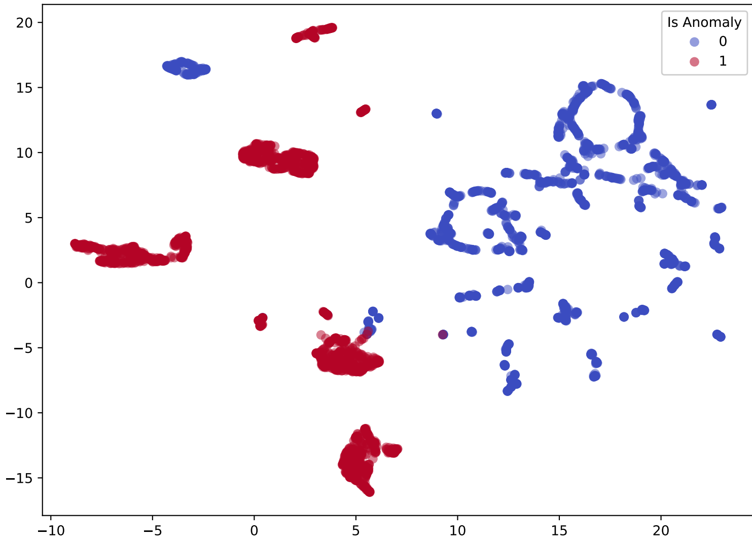
UMAP Projection
