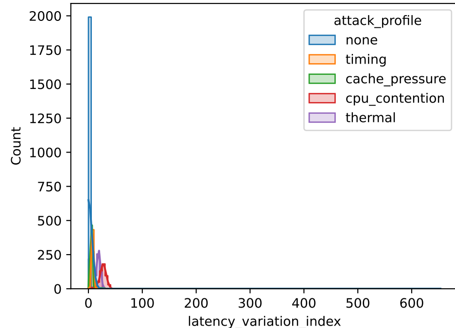
Distribution: latency_variation_index
