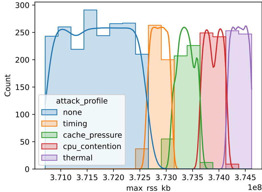
Distribution: max_rss_kb
