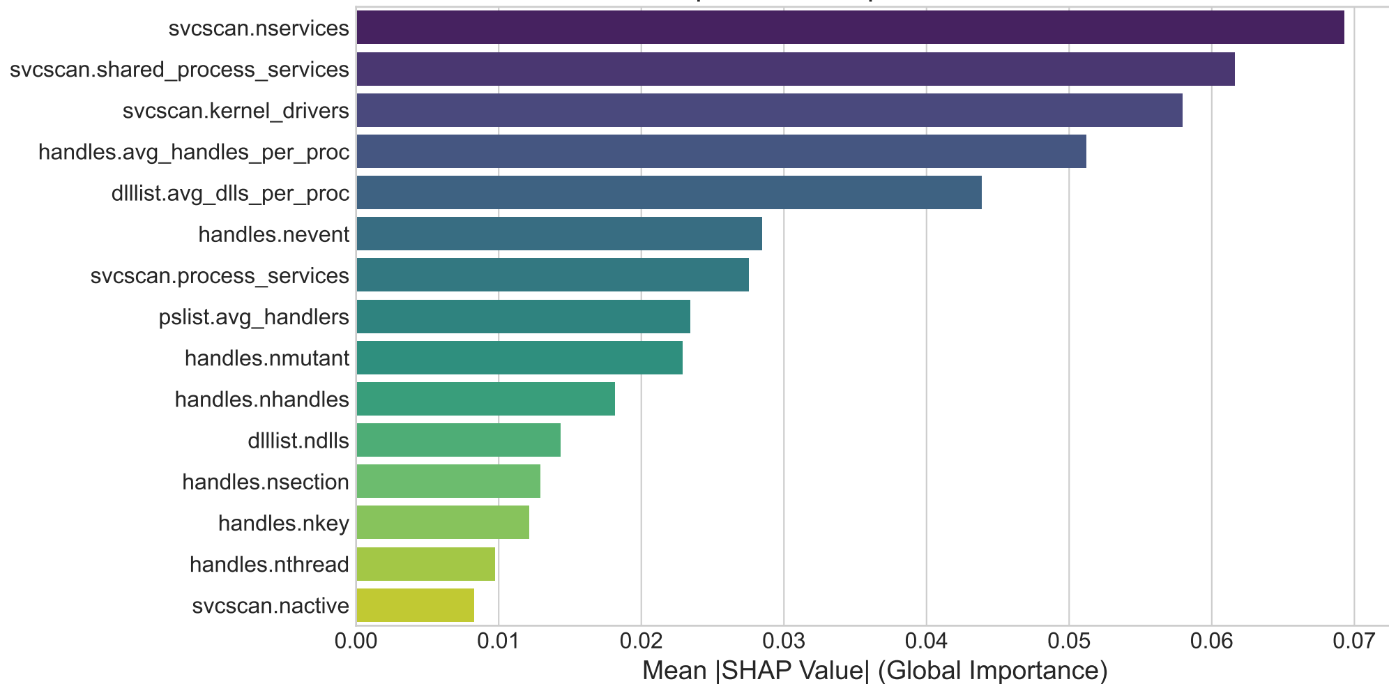
Top 15 Most Important Features
